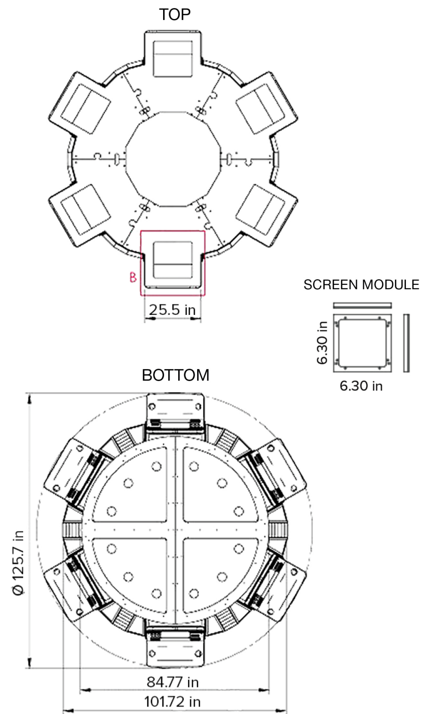
DIMENSION 49J Pod-of-6
