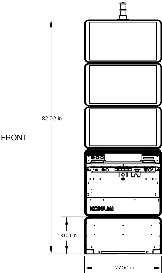
DIMENSION 27 Single Cabinet
