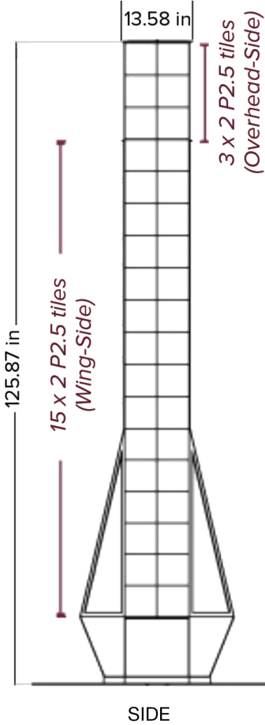
DIMENSION 49J Bank-of-6
