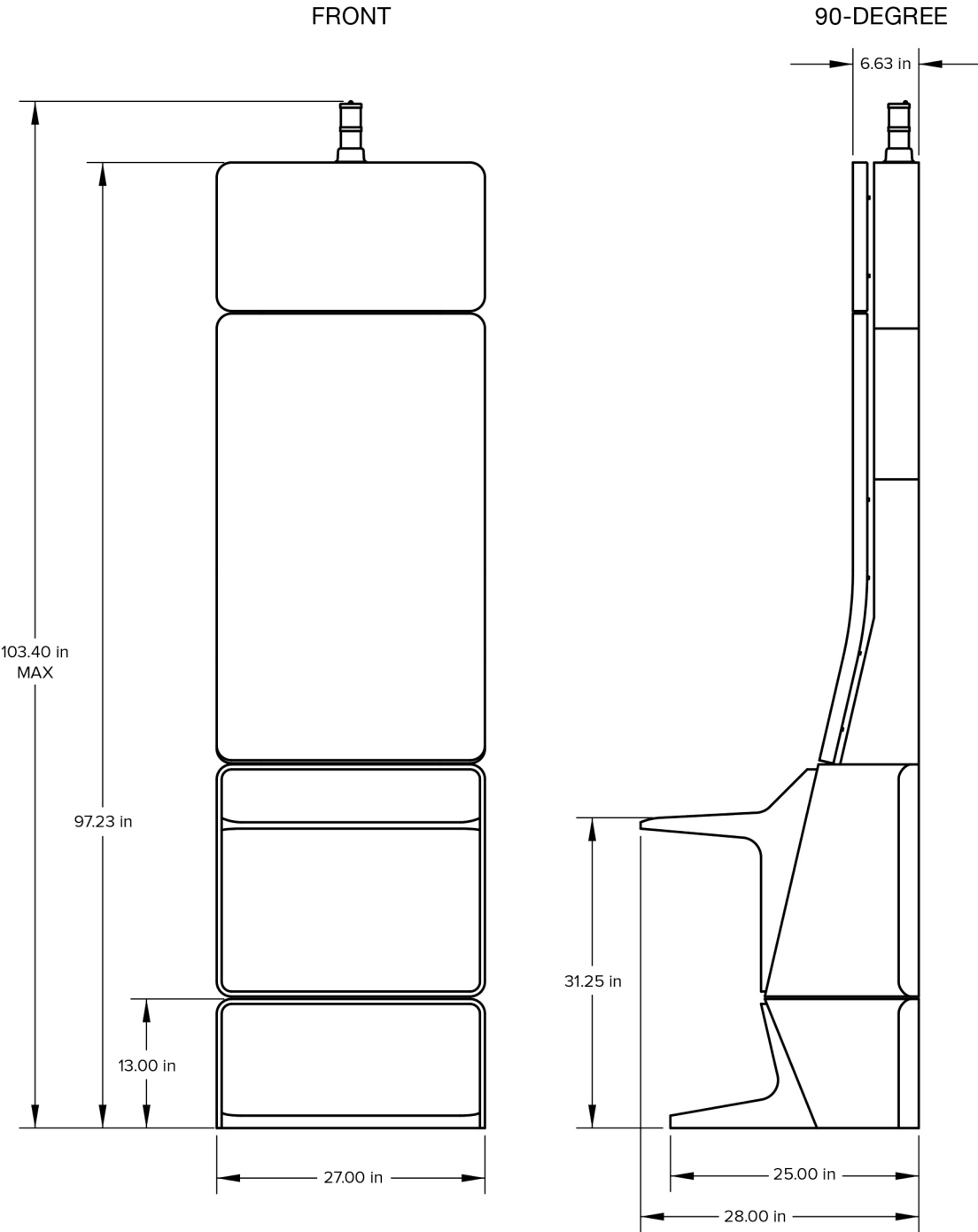
DIMENSION 49J Single Cabinet
