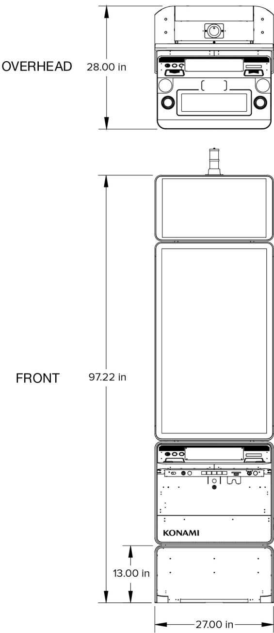
DIMENSION 49 Single Cabinet
